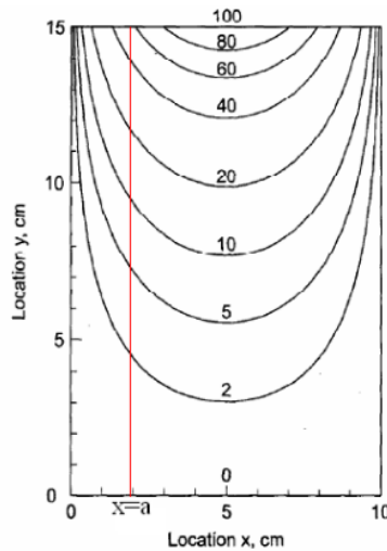
Figure 2.1.1: A metallic bar
