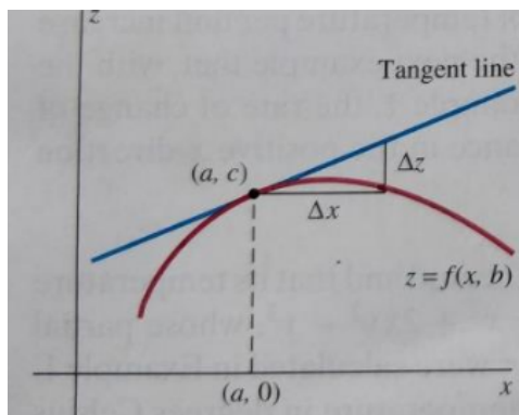
Figure 2.3.3: The tangent to the curve z = f(x, b)
